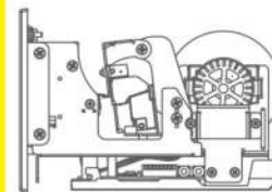
SP1-BDS- With Anti-drag
