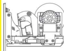
SP1-BNS- Without Anti-drag
